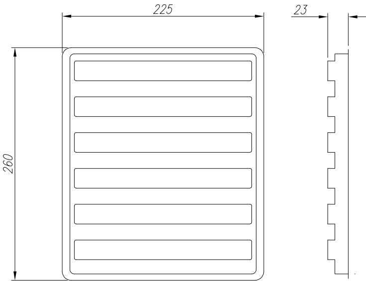
UPPER COVER
