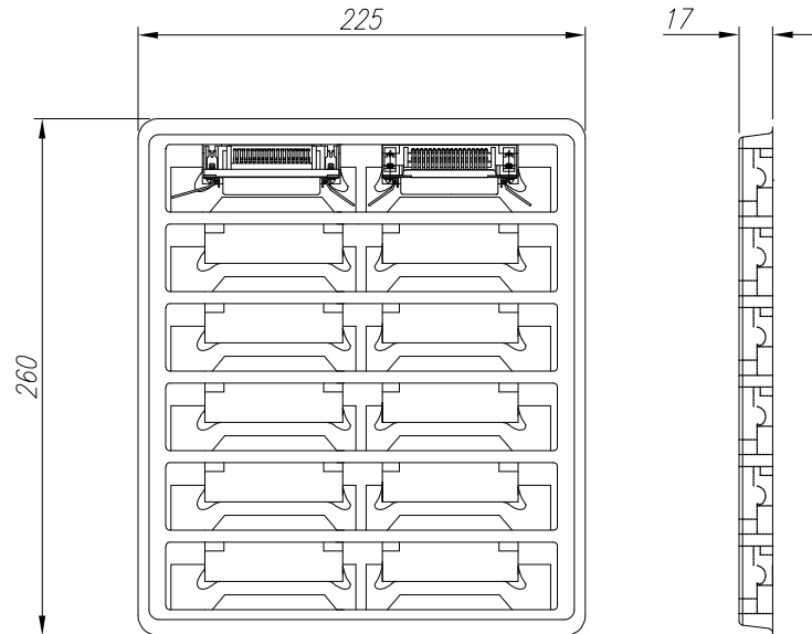
LOWER COVER
