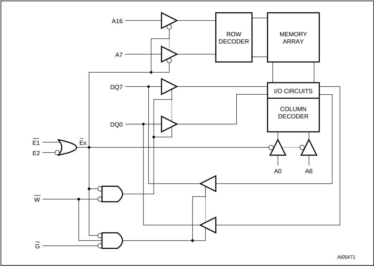
Figure 5. Block Diagram
