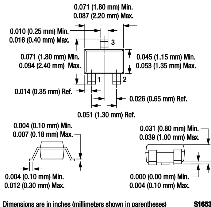
Figure 7. SC-70 Package Dimension Drawing
