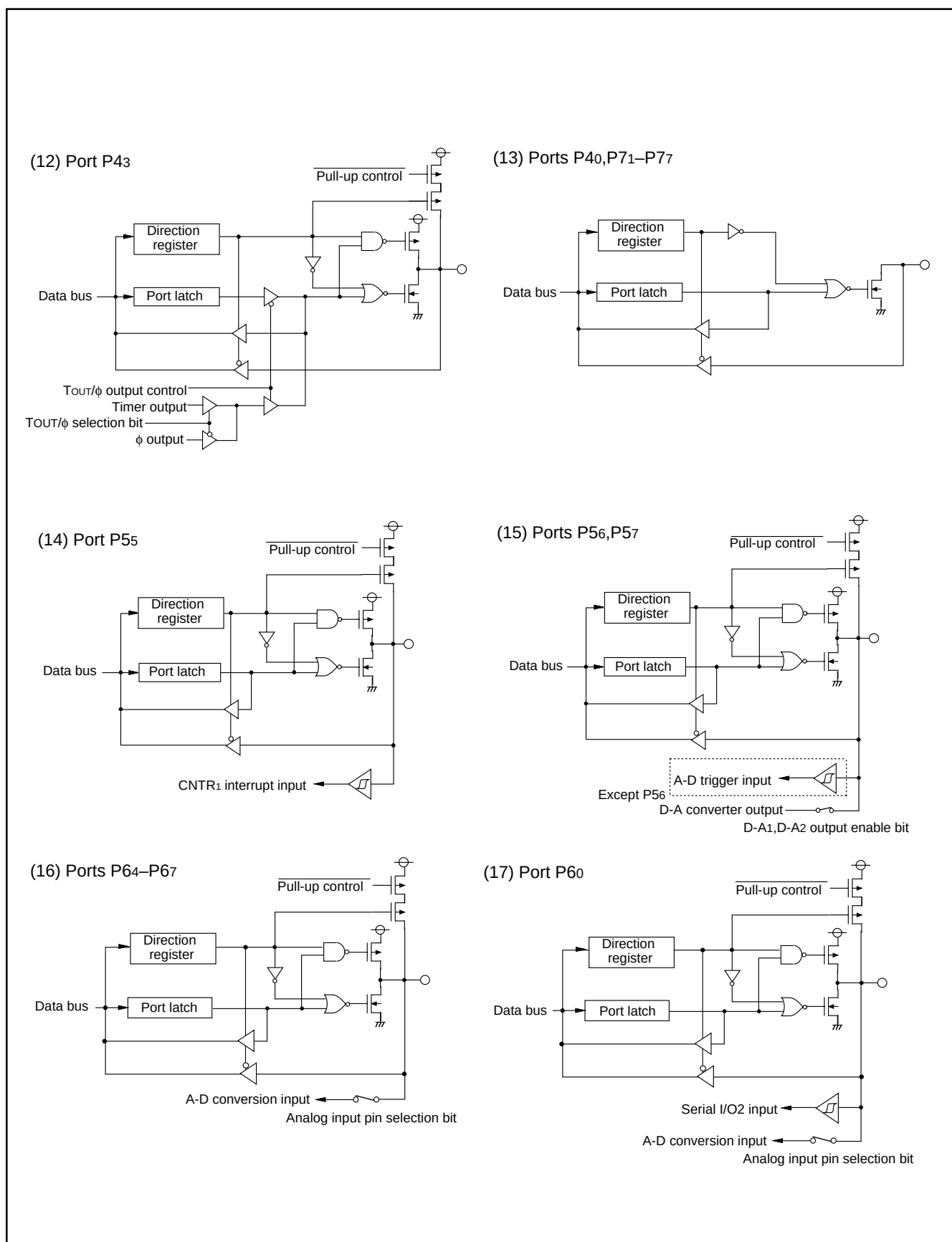
Fig. 15 Port block diagram (3)
