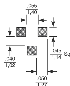
Land Pattern
