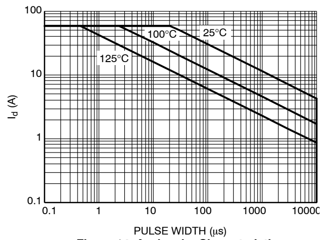
Figure 14. Avalanche Characteristics
