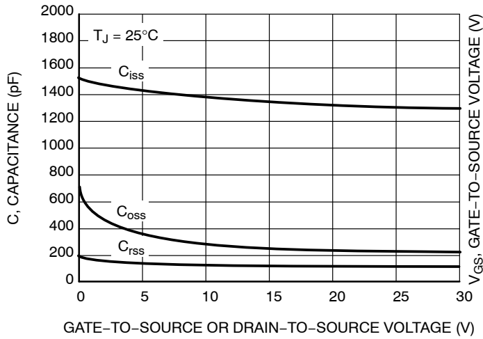
Figure 7. Capacitance Variation
