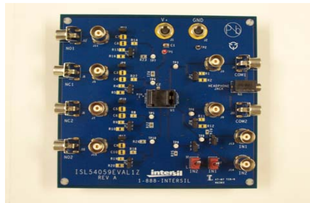
FIGURE 1. ISL54059EVAL1Z THROUGH ISL54064EVAL1Z EVALUATION BOARD
