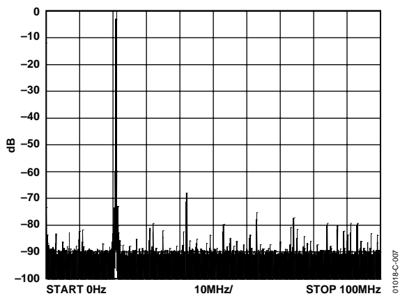
Figure 7. 21 MHz Single-Tone Output
