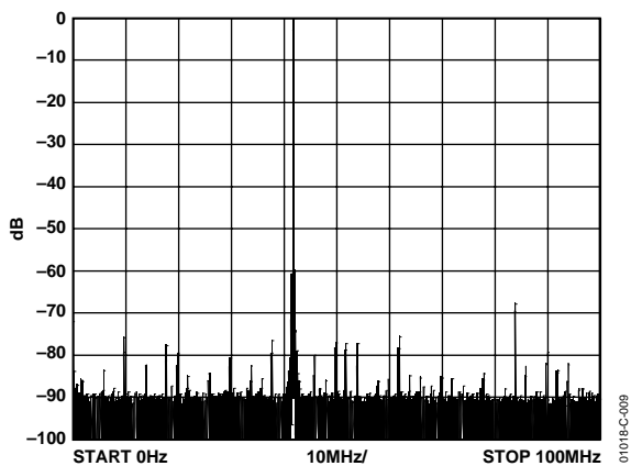
Figure 9. 42 MHz Single-Tone Output
