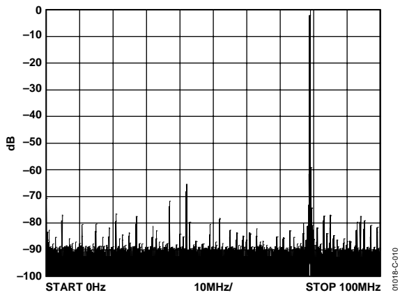
Figure 10. 79 MHz Single-Tone Output
