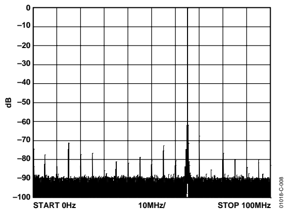
Figure 8. 65 MHz Single-Tone Output
