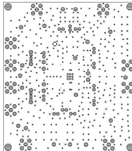
Figure 123. Ground Plane
