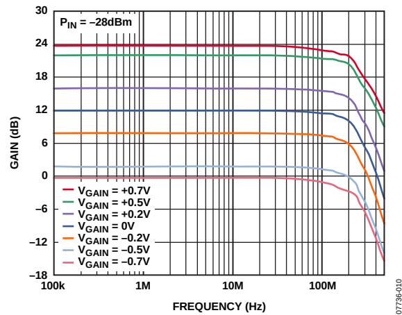
Figure 10. Frequency Response vs. Gain to V_{GA} for Various Values of V_{GA}
