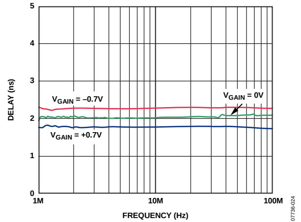
Figure 24. Group Delay vs. Frequency to VGAX
