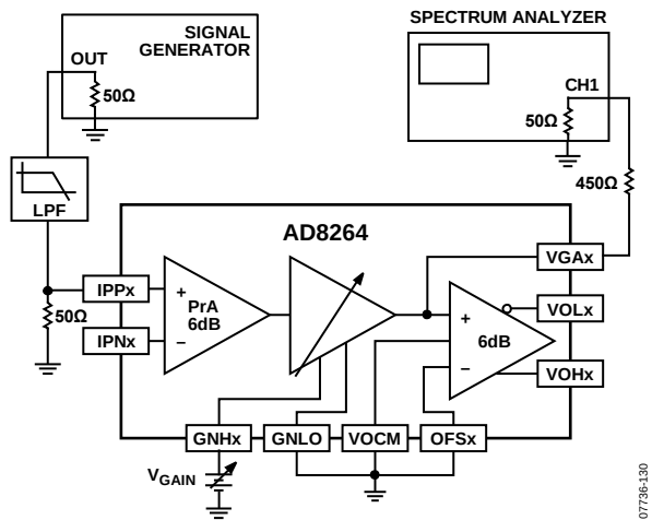
Figure 94. HD2 and HD3 to VGAX (See Figure 42 Through Figure 45)
