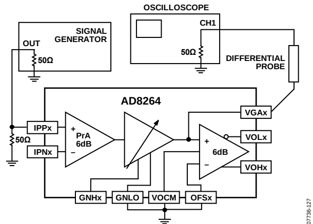
Figure 108. VGA Overdrive Recovery, V_{GAIN} = 0.7\text{ V} (See Figure 67)
