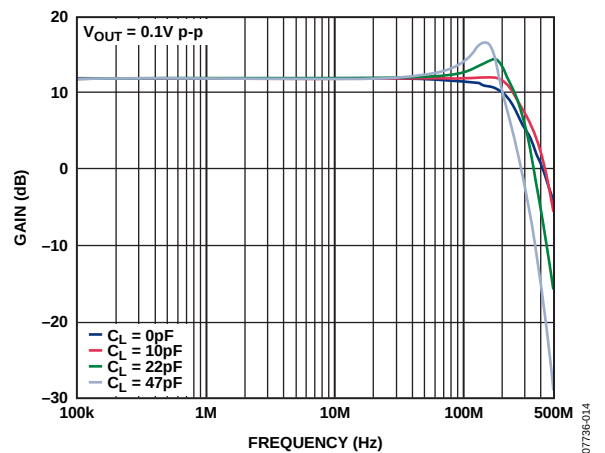
Figure 14. Small Signal Frequency Response to V_{GA} for Various Capacitive Loads
