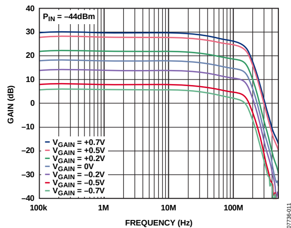
Figure 11. Frequency Response vs. Gain to Differential Output for Various Values of V_{GA}
