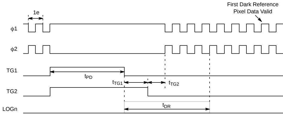
Figure 17. Photodiode-to-CCD Transfer
