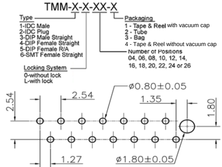
PCB Layout
