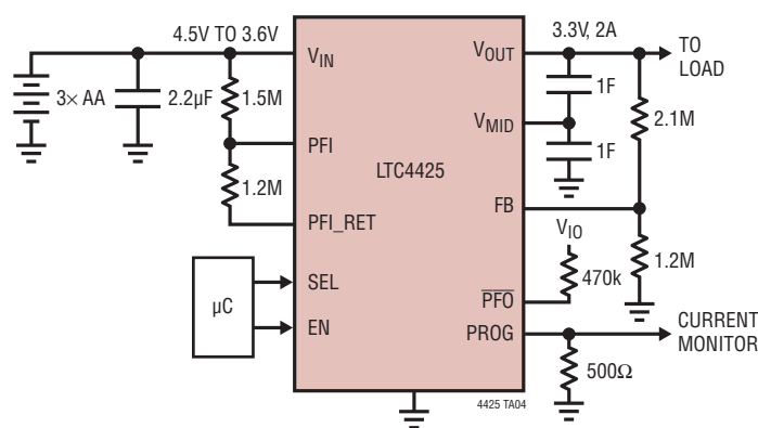
3 × AA Alkaline to High Peak Power 3.3V Charging
