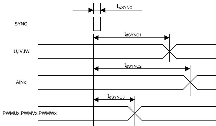
Figure 8. SYNC timing
