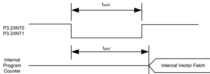
Figure 11. Interrupt timing
