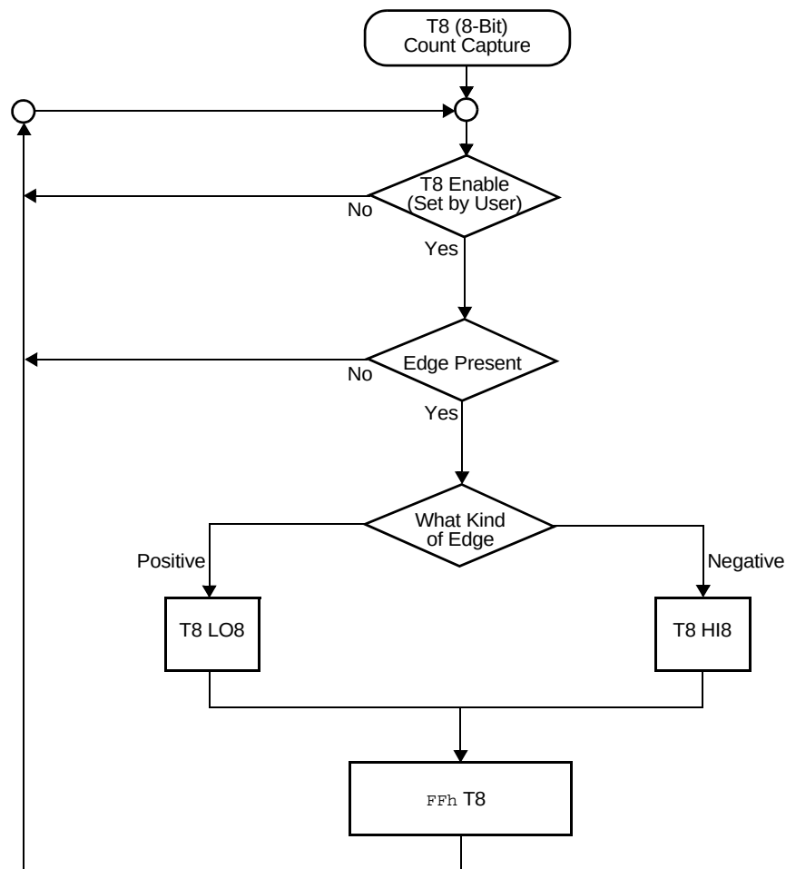
Figure 20.DEMODULATION Mode Count Capture Flowchart
