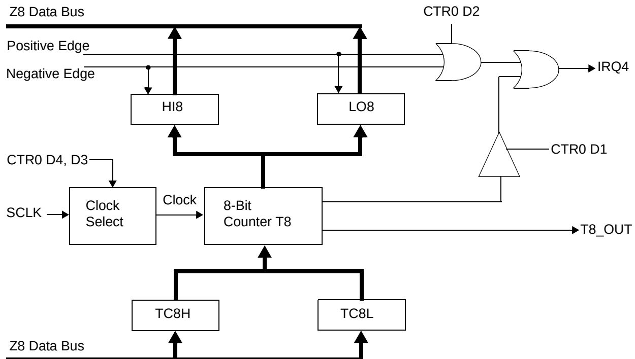
Figure 17.8-Bit Counter/Timer Circuits
