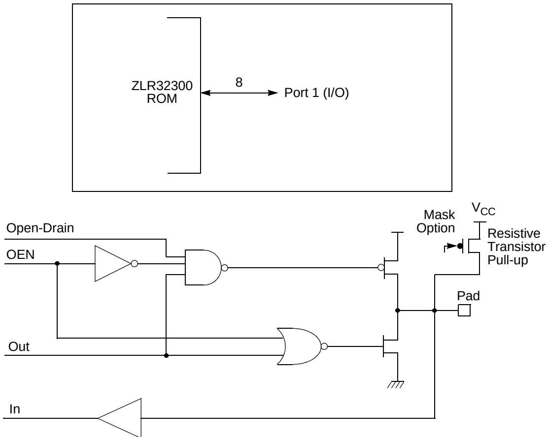
Figure 7. Port 1 Configuration
