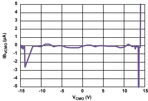
FIGURE 16. IB_{VCM0} vs V_{CM0} INPUT VOLTAGE RANGE
