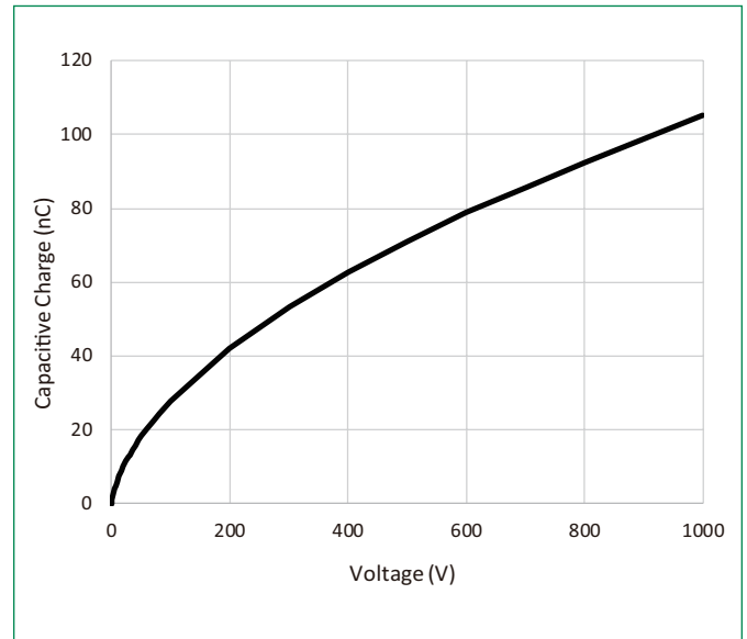
Figure 6: Capacitive Charge vs. Reverse Voltage (Per Leg)
