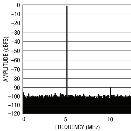
LTC2263-12: 8k Point FFT, f_{IN} = 5\text{MHz} , -1\text{dBFS} , 25Msps
