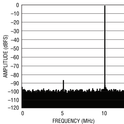
LTC2263-12: 8k Point FFT, f_{IN} = 140\text{MHz} , -1\text{dBFS} , 25Msps
