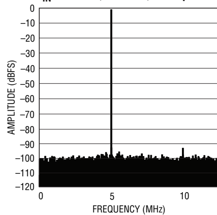
LTC2263-12: 8k Point FFT, f_{IN} = 30\text{MHz} , -1\text{dBFS} , 25Msps
