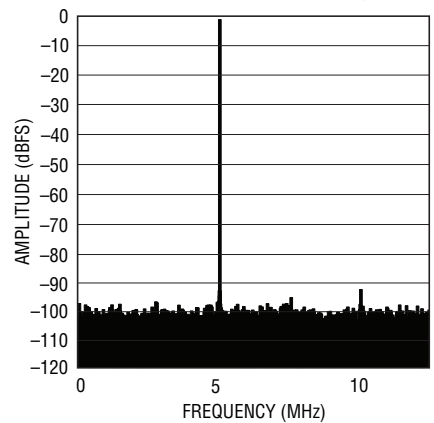
LTC2263-12: 8k Point FFT, f_{IN} = 70\text{MHz} , -1\text{dBFS} , 25Msps
