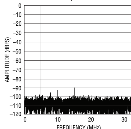
LTC2265-12: 8k Point FFT, f_{IN} = 5\text{MHz} , -1dBFS, 65Msps
