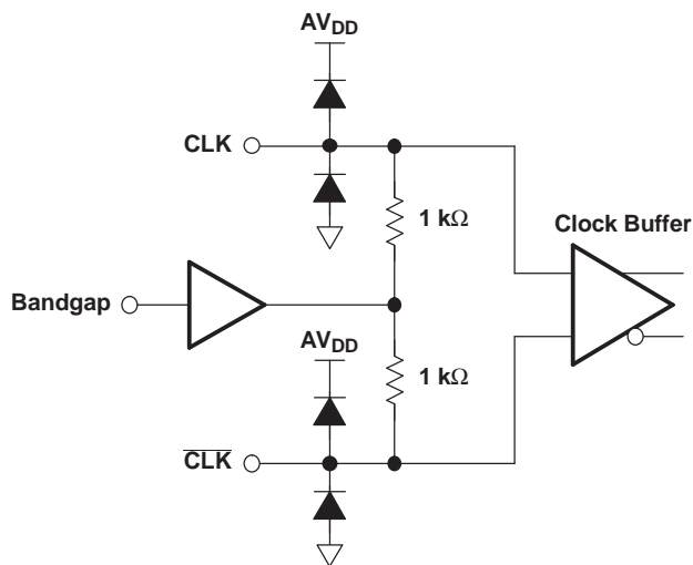
Figure 29. Clock Input
