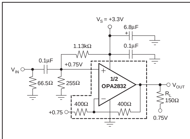
Figure 62. AC-Coupled, G = +2, +3V Single-Supply Specification and Test Circuit
