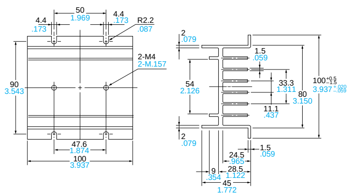
Mounting dimensions
