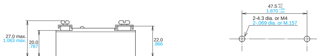
Mounting dimensions
