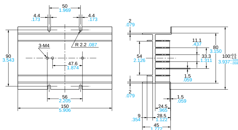
Mounting dimensions
