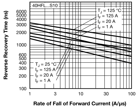
Fig. 23 - Typical Reverse Recovery Time vs. Rate of Fall of Forward Current, 40HFL...Series
