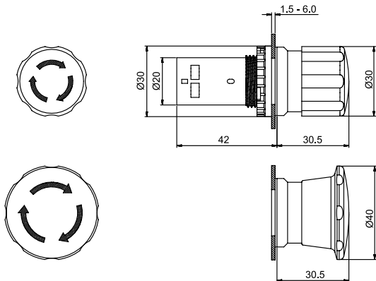
CE3T/CE4T (Twist release)
