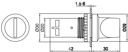
Selector Switch
