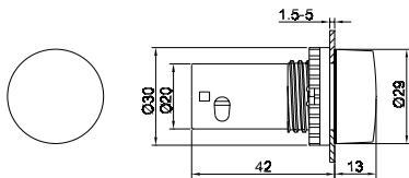
Pilot Light
