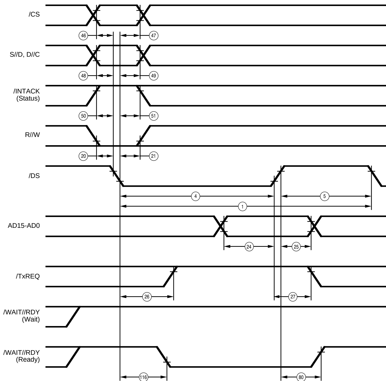
Figure 90. Non-Multiplexed /DS Write Cycle
