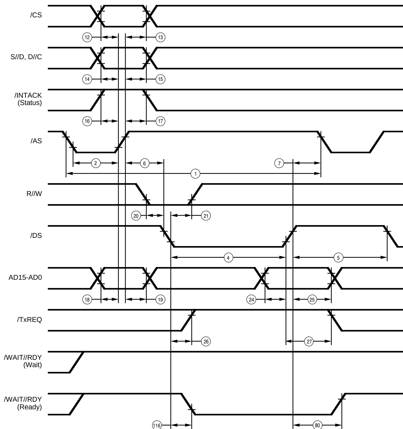
Figure 86. Multiplexed /DS Write Cycle
