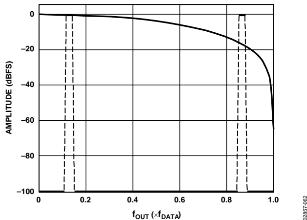
Figure 62. No Interpolation, Modulation = f_{DAC}/8
