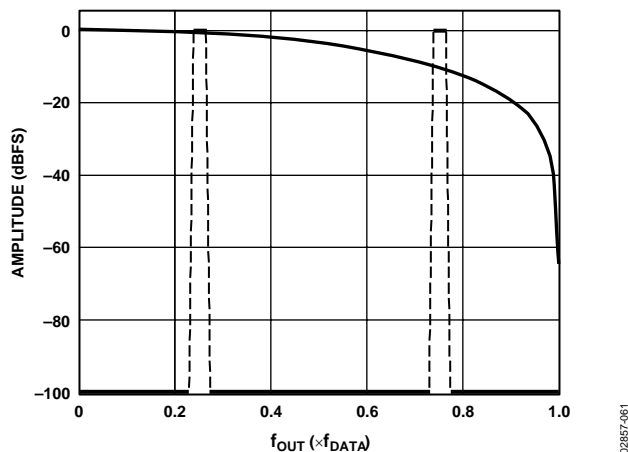
Figure 61. No Interpolation, Modulation = f_{DAC}/4
