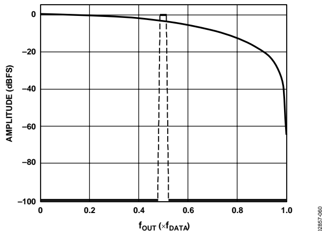
Figure 60. No Interpolation, Modulation = f_{DAC}/2
