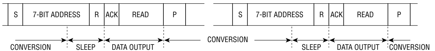
Figure 7. Consecutive Reading with the Same Input/Configuration
