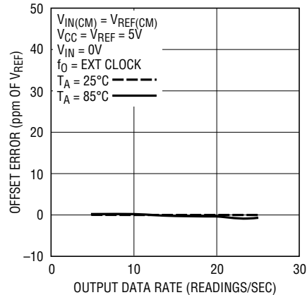
Figure 30. Offset Error vs Output Data Rate and Temperature
