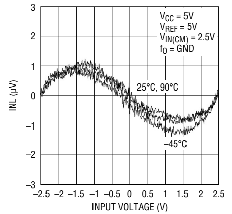
Integral Nonlinearity (2x Speed Mode; V_{CC} = 5\text{V} , V_{REF} = 5\text{V} )
