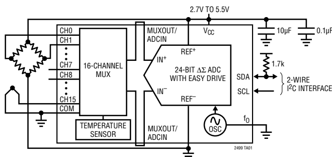
Data Acquisition System with Temperature Compensation
