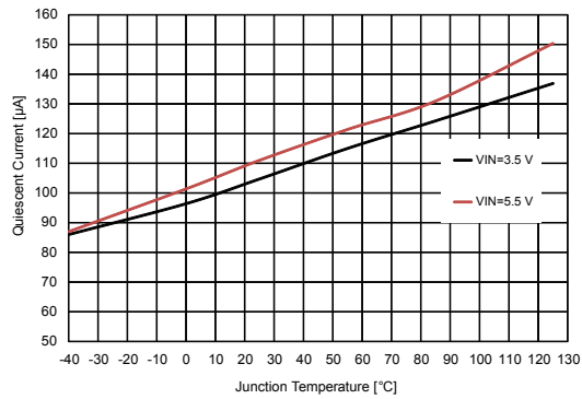
Figure 8. Quiescent current vs. temperature ( V_{OUT} = 3.0\text{ V} , I_{OUT} = 0\text{ mA} )
