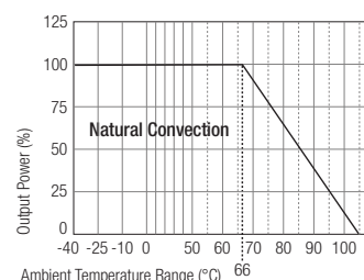
RP15-4805SAW With Heat Sink
