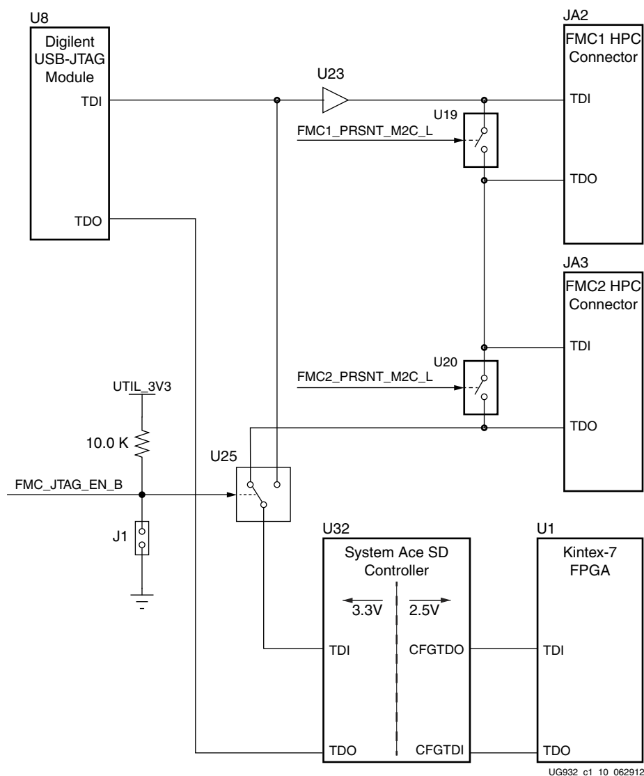
Figure 1-10: JTAG Chain
