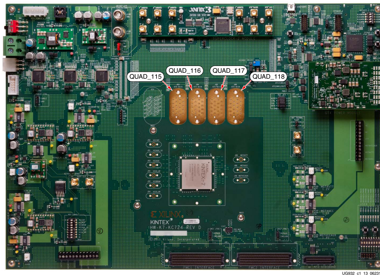
Figure 1-13: GTX Quad Locations
