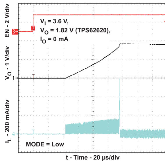
Figure 10. TPS62620EVM Start-Up
