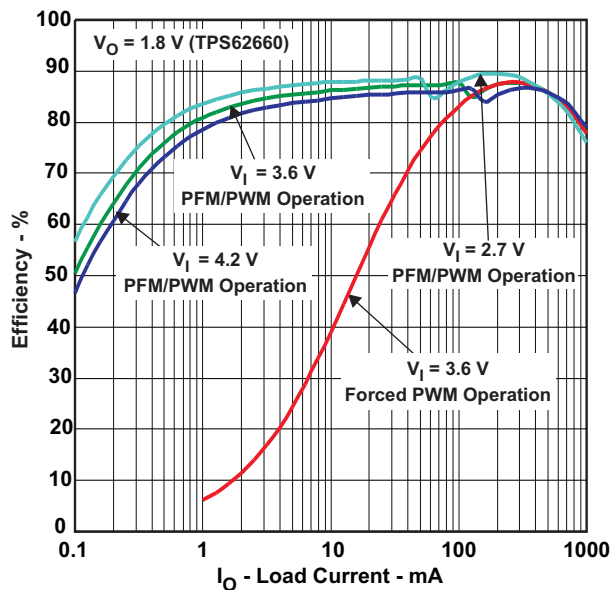
Figure 7. TPS6266xEVM Efficiency versus Load Current ( V_{OUT} = 1.8 V)
