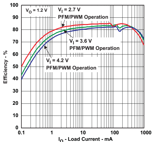
Figure 8. TPS6266xEVM Efficiency versus Load Current ( V_{OUT} = 1.2 V)
