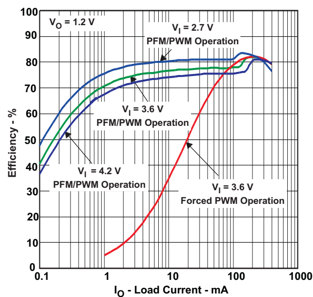
Figure 6. TPS6261xEVM Efficiency versus Load Current ( V_{OUT} = 1.2\text{ V} )
