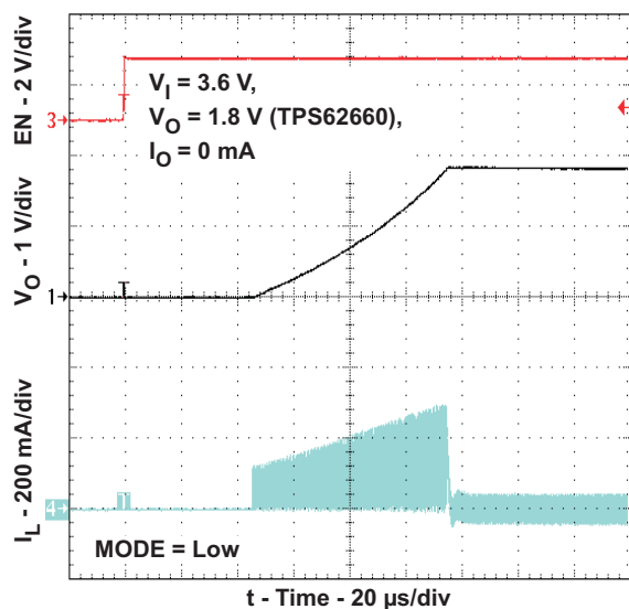
Figure 9. TPS62660EVM Startup
