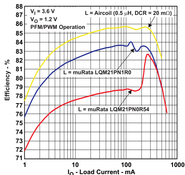
Figure 4. TPS6262x and TPS6262xEVM Efficiency versus Load Current ( V_{IN} = 3.6\text{ V} )
