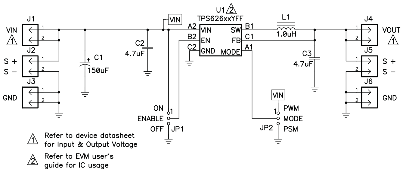
Figure 1. TPS626xxEVM Schematic
