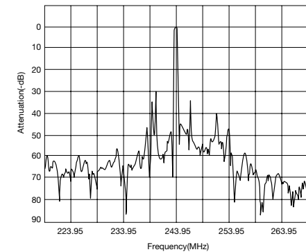
PAFC243B Spurious Characteristics
