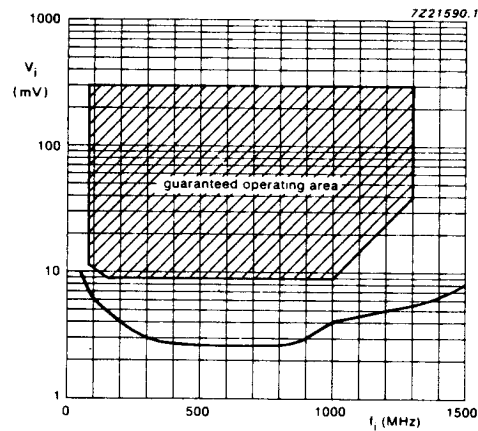
Fig.6 Prescaler typical input sensitivity curve; V_{CC} = 4.5 to 5.5 V; T_{amb} = -10 to +80 °C.
