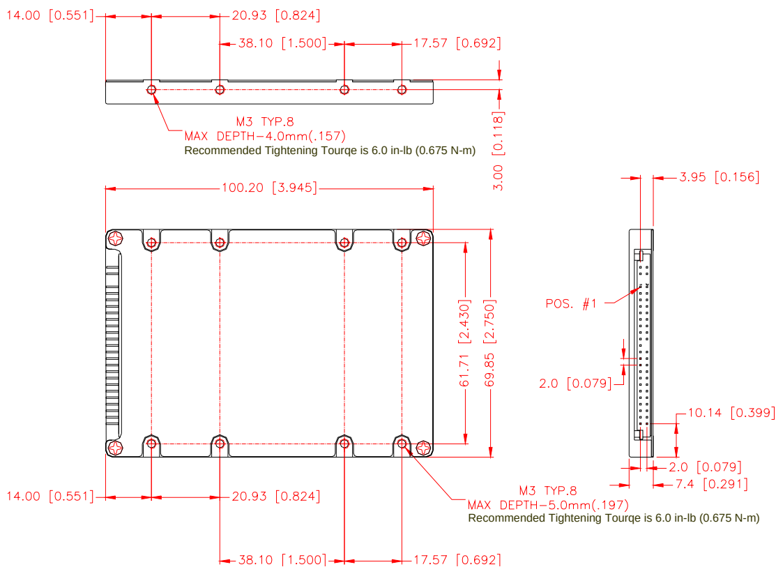
Figure 2: IDE 4000 2.5" Assembly
