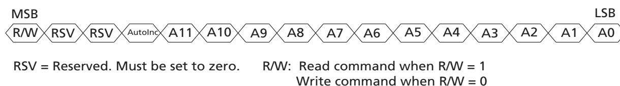
Figure 3-13: Command Word Format
