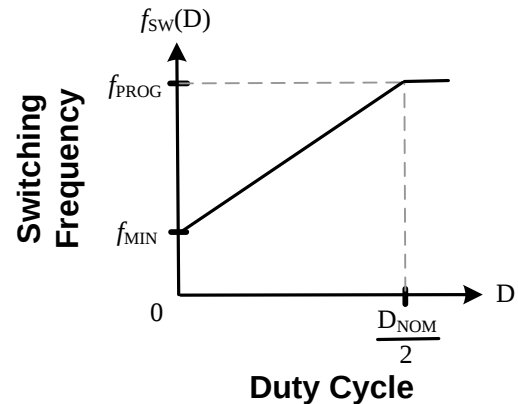
Figure 16. Adaptive Frequency
