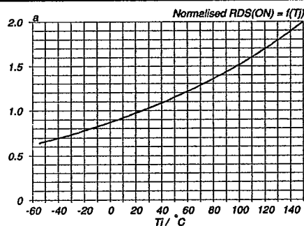
Fig. 9. Normalised drain-source on-state resistance. a = R_{DS(ON)}/R_{DS(ON)25^\circ C} = f(T_j) ; I_D = 15 A; V_{GS} = 10 V
