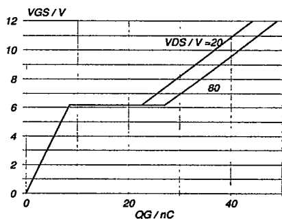
Fig. 13. Typical turn-on gate-charge characteristics. V_{GS} = f(Q_G) ; conditions: I_D = 33 \text{ A} ; parameter V_{DS}
