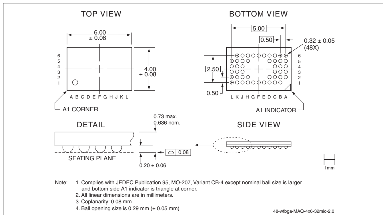
FIGURE 27: 48-ball Very-Very-Thin-Profile, Fine-pitch Ball Grid Array (WFBGA) 4mm x 6mm SST Package Code MAQ
