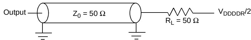
Figure 10. DDR AC Test Load
