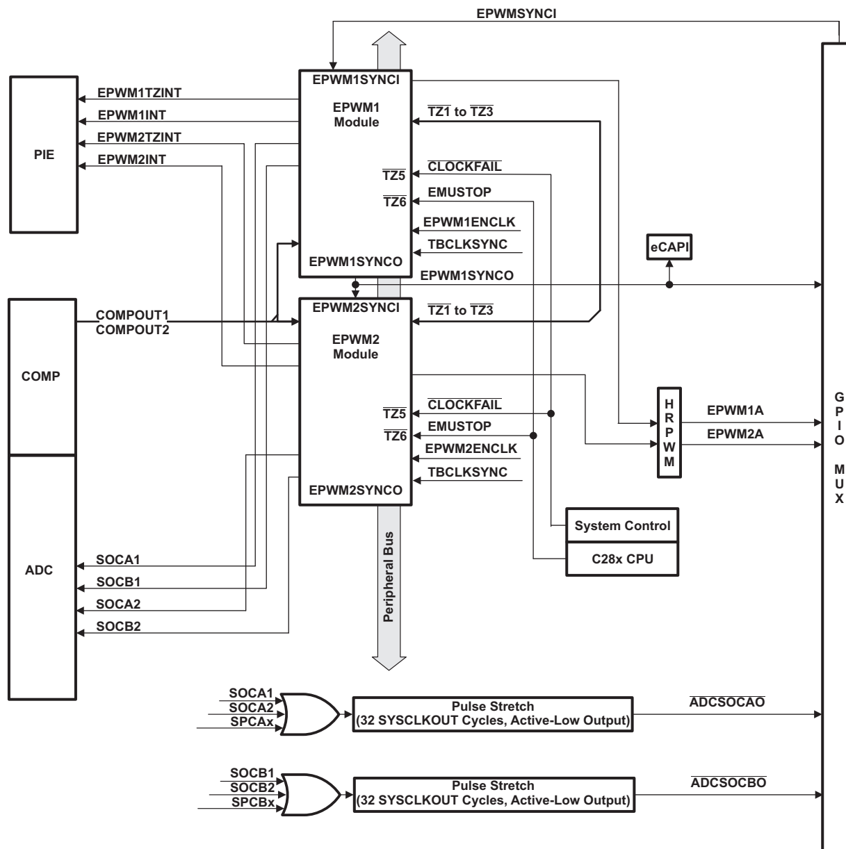
Figure 5-38. ePWM
