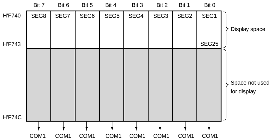
Figure 13.6 LCD RAM Map (Static Mode)
