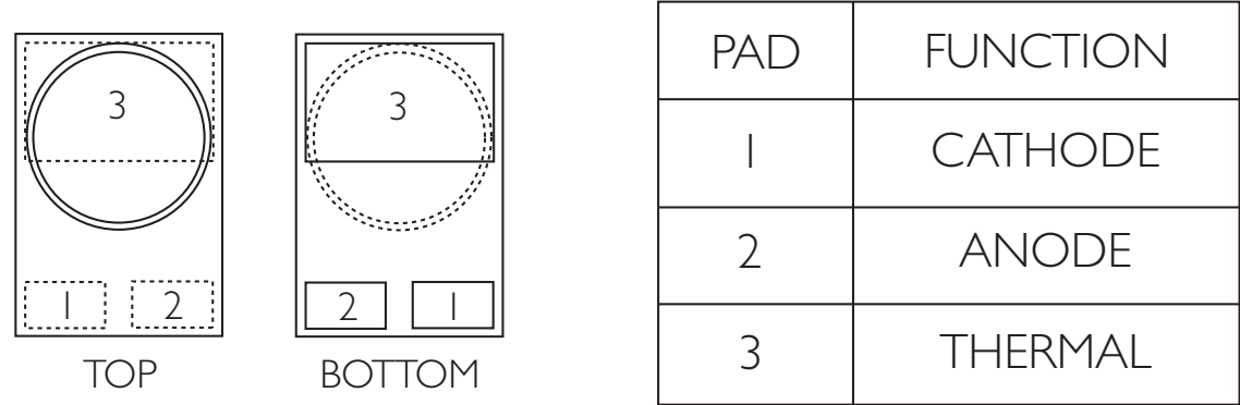
Figure 2. Pad configuration.
