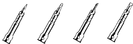
WPT-01 10 mm Taper Needle WPT-02 2.4 mm Chisel WPT-03 2.0 mm Spade WPT-04 5.0 mm Chisel
