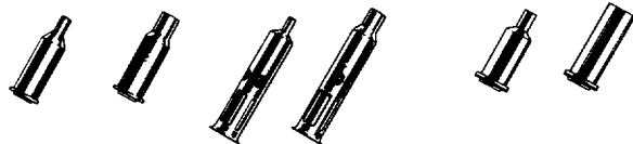
WHC-50 1.5 mm Diameter WHC-52 4.9 mm Diameter WHC-54 1.5 mm Diameter WHC-55 4.7 mm Diameter WHC-57 3.6 mm Diameter WHC-58 9.7 mm Diameter
