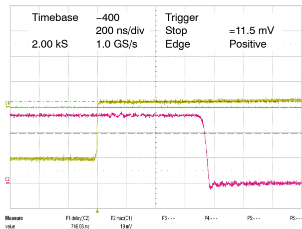
Figure 10. 10 mV Overdrive
