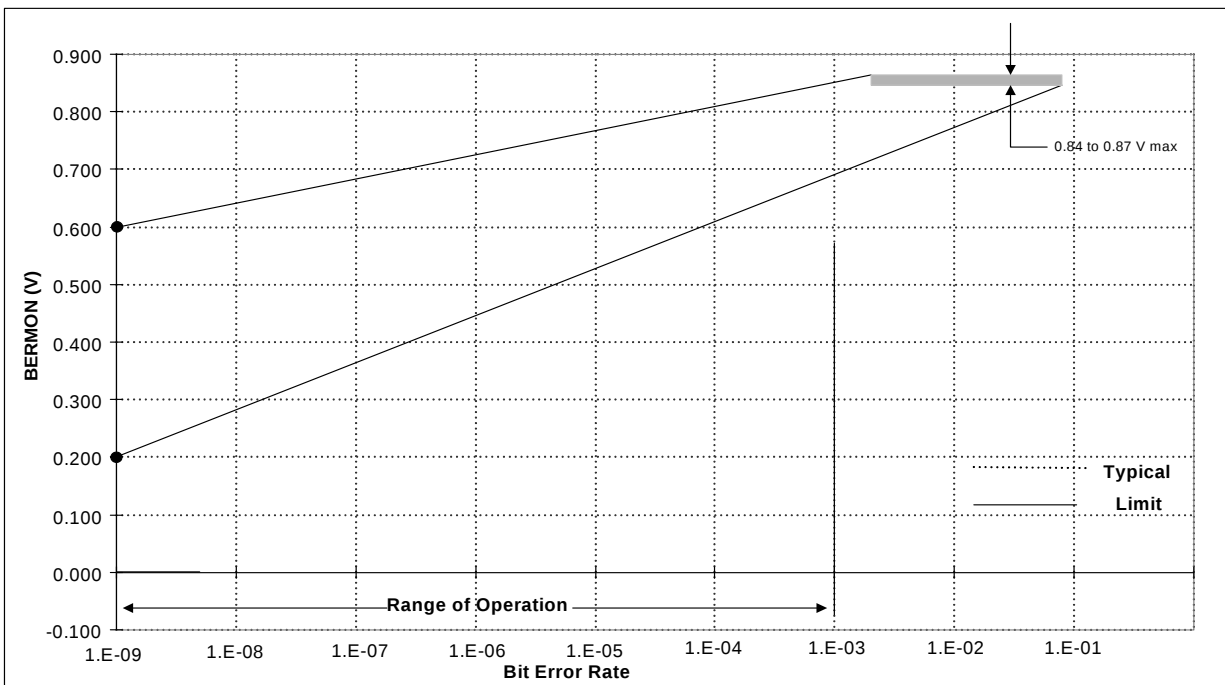
Figure 8. Si5023 OC-48 BERMON Voltage Characteristics
