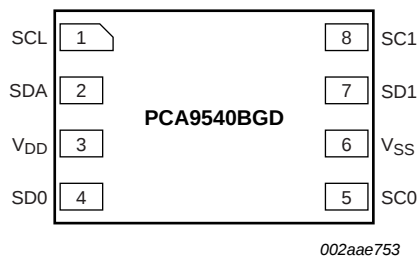
Fig 4. Pin configuration for XSON8
