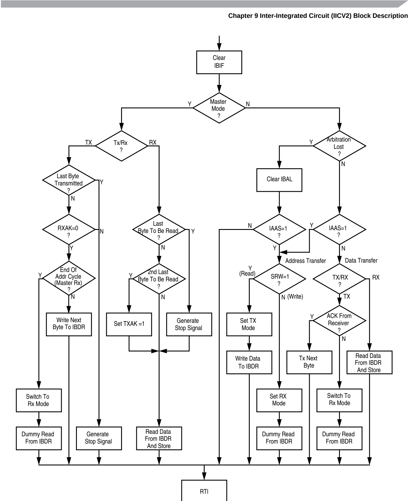
Figure 9-12. Flow-Chart of Typical IIC Interrupt Routine
