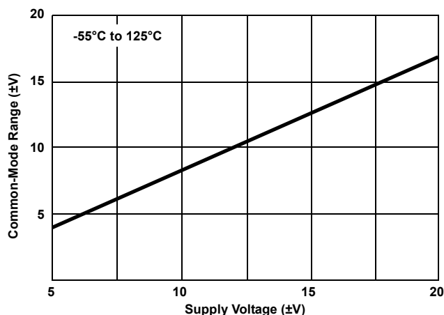
Figure 14. Common-Mode Voltage Range vs Supply Voltage
