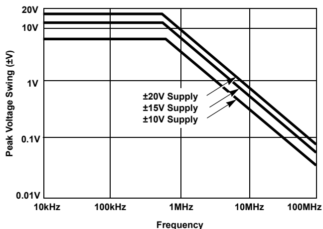
Figure 12. Output Voltage Swing vs Frequency
