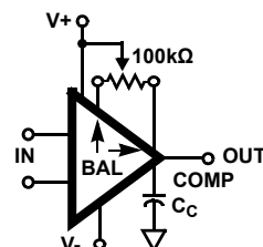
Figure 7. Suggested V_{OS} Adjustment and Compensation Hook-Up
