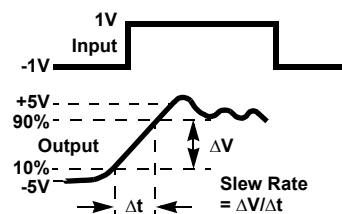
Figure 5. Slew Rate
