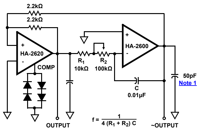
Figure 2. Function Generator
