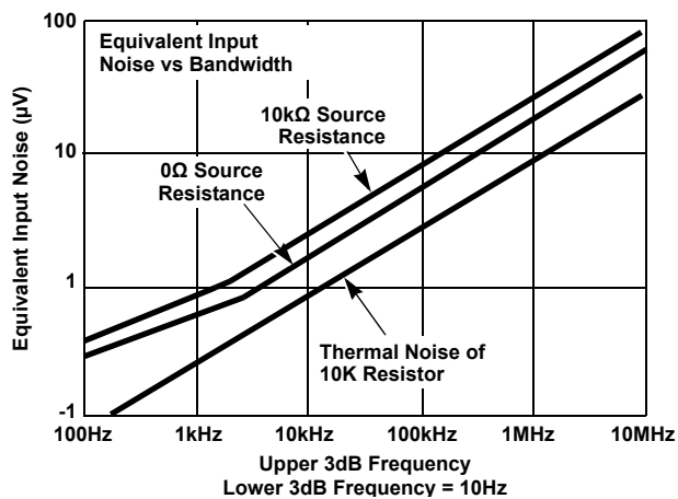
Figure 9. Broadband Noise Characteristics
