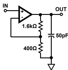
Figure 6. Slew Rate and Transient Response
