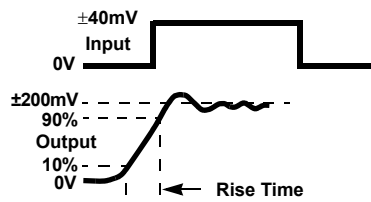
Figure 4. Transient Response
