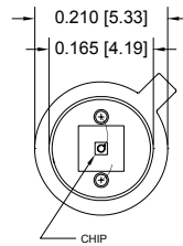
CHIP DIMENSIONS INCH [mm]
