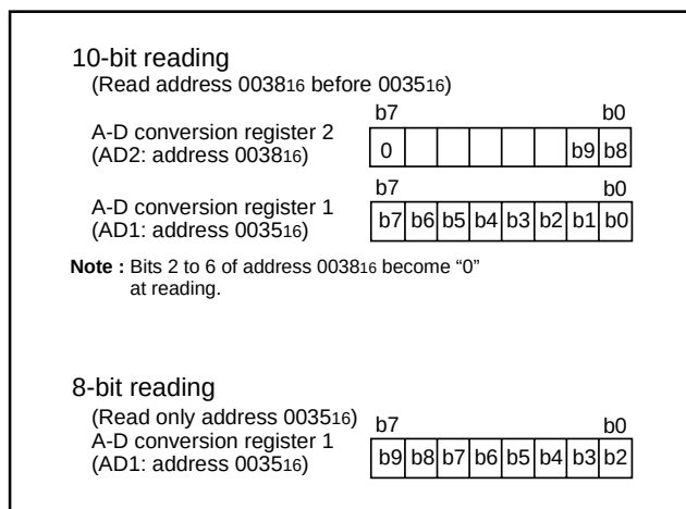
Fig. 58 Structure of 10-bit A-D mode reading
