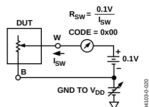
Figure 32. Test Circuit for Incremental On Resistance
