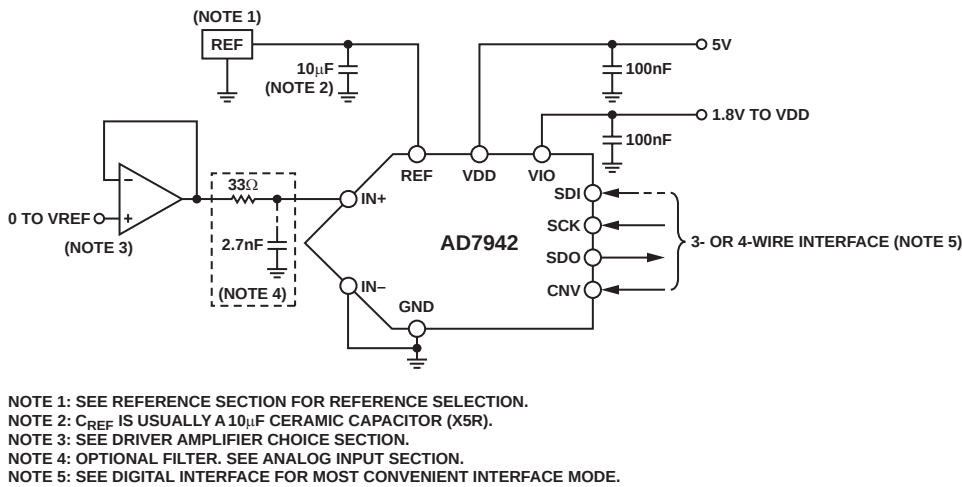
Figure 22. Typical Application Diagram with multiple supplies
