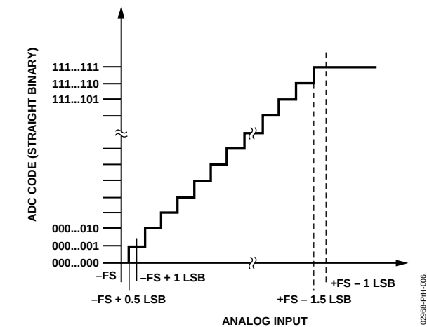
Figure 21. ADC Ideal Transfer Function
